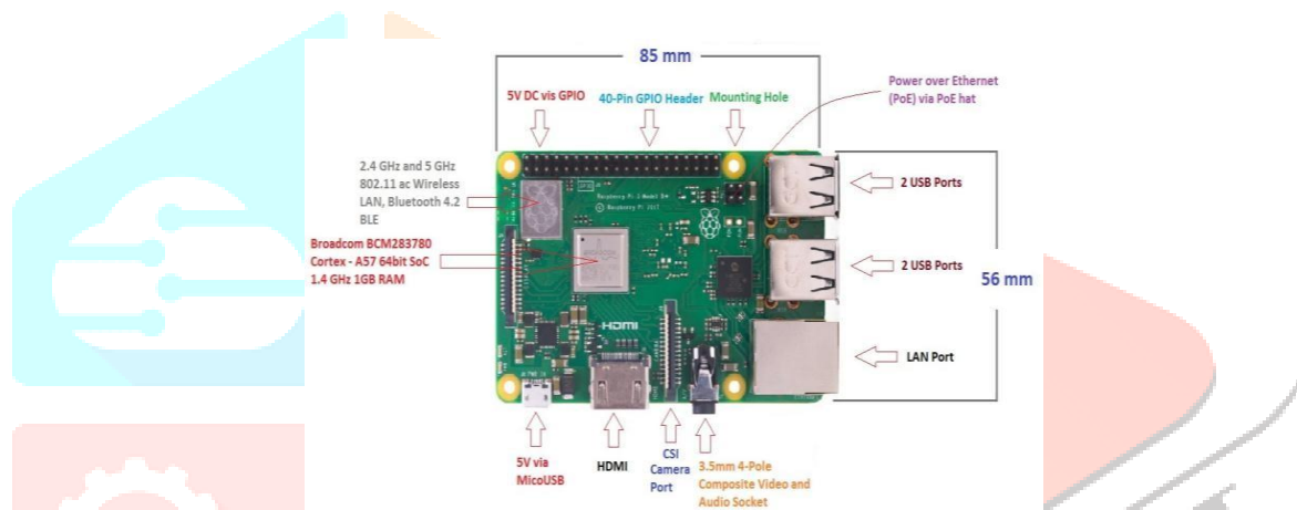
Fig: Raspberry Pi 3 Model B+
