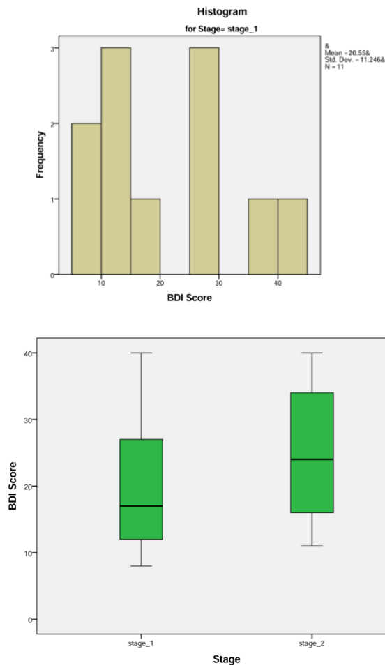
BDI Score Histograms
