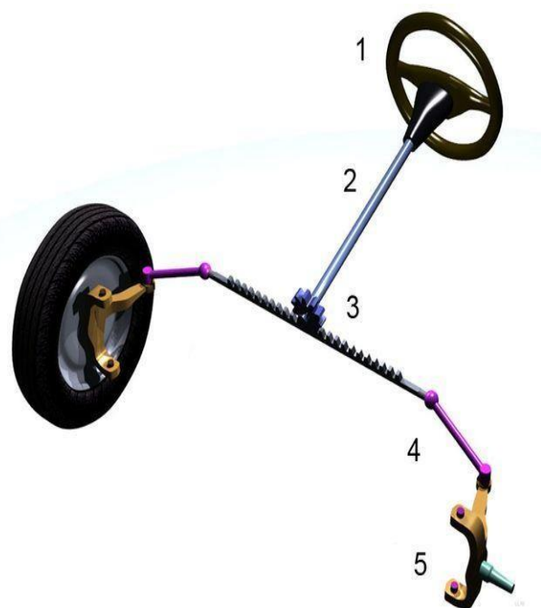
Fig:1. 2 Rack and pinion steering geometry
