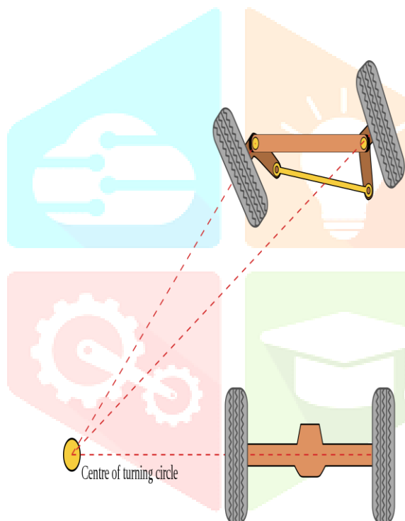
Fig: 1.1 Ackermann steering geometry
