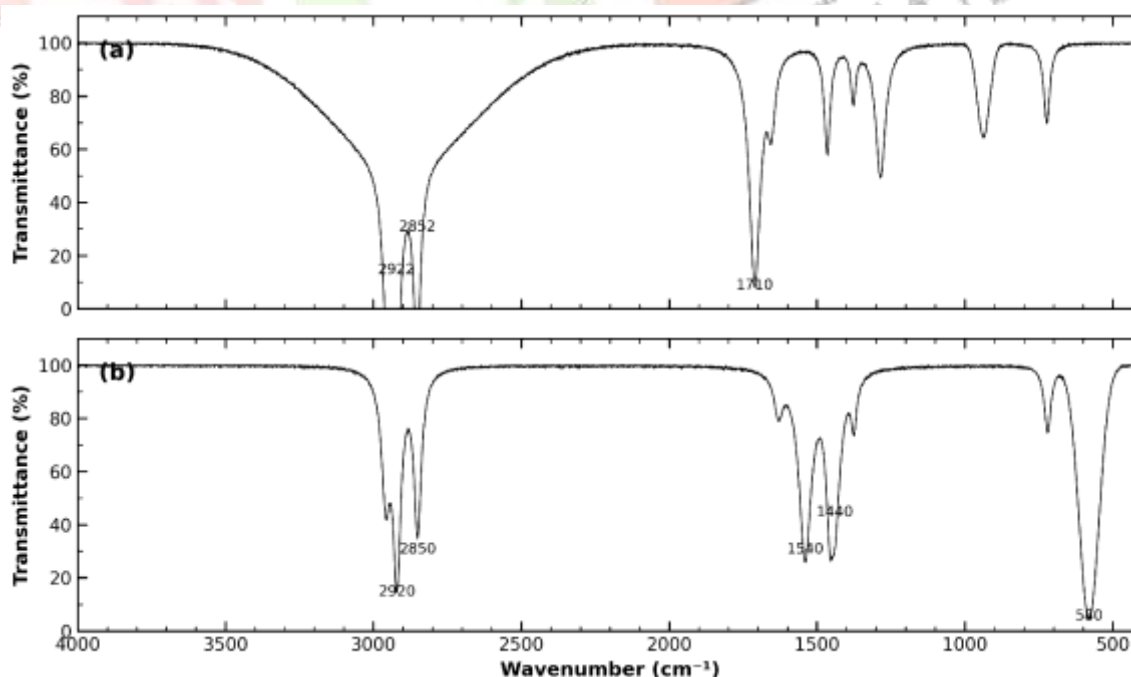
Figure 5. FTIR spectra of (a) pure oleic acid and (b) oleic acid-coated \text{Fe}_3\text{O}_4 nanoparticles, highlighting \text{COO}^- asymmetric ( \sim 1540\text{ cm}^{-1} ) and symmetric ( \sim 1440\text{ cm}^{-1} ) stretching vibrations.
