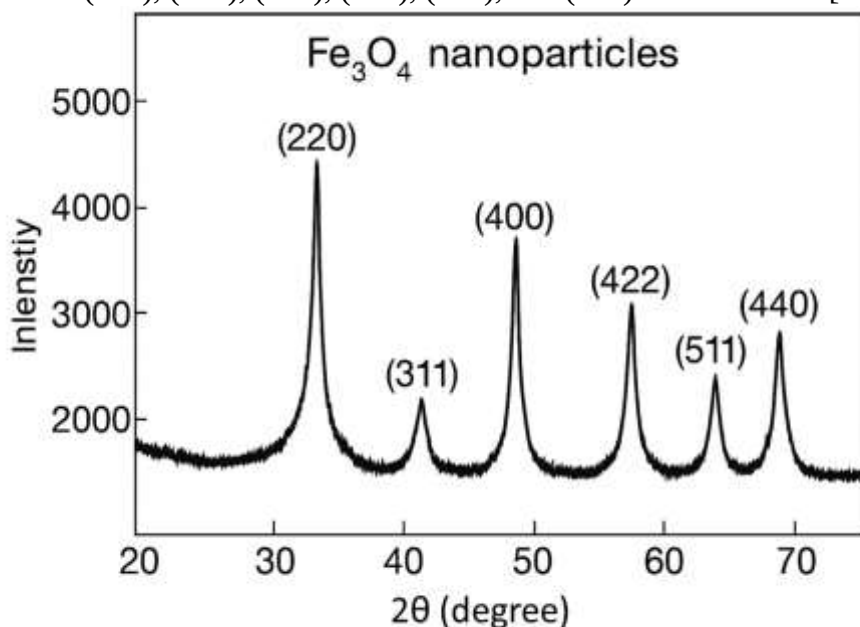
Figure 3. Representative XRD pattern of \text{Fe}_3\text{O}_4 nanoparticles showing diffraction peaks corresponding to (220), (311), (400), (422), (511), and (440) planes of the spinel structure.
