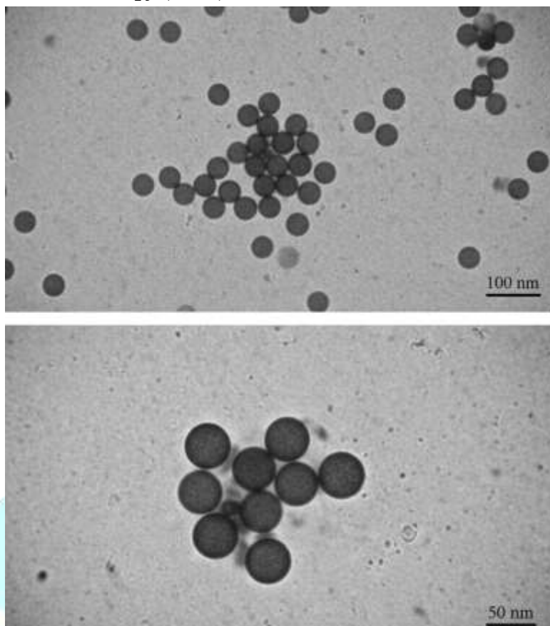
Figure 4. TEM images of oleic acid-coated \text{Fe}_3\text{O}_4 nanoparticles showing uniform spherical morphology and narrow size distribution.
