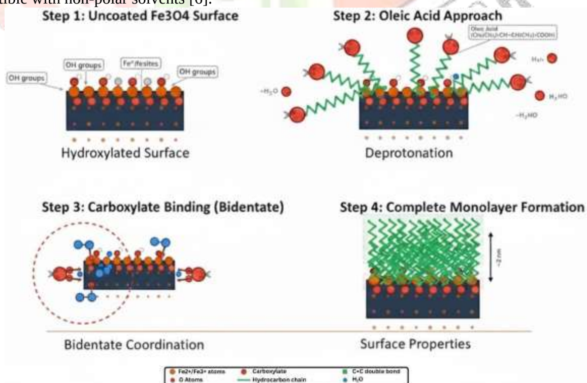
Figure 2. Stepwise schematic representation of oleic acid coating on Fe_3O_4 nanoparticles showing carboxylate bonding to surface Fe^{2+}/Fe^{3+} sites and hydrophobic tail orientation
