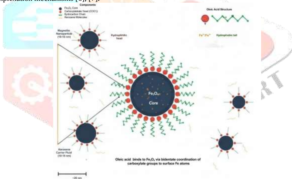
Figure 1. Structure of a ferrofluid showing \text{Fe}_3\text{O}_4 nanoparticles coated with oleic acid dispersed in a kerosene carrier
